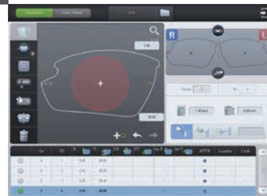
Hole Editor
